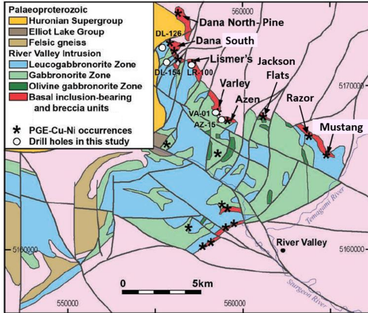
Geological map of River Valley Property area (adapted from Holwell et al., 2014)
