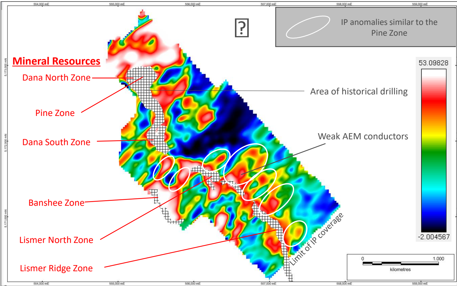
Colour image of 2018 merged IP chargeability surveys at 250 m level (approx. 70 m below surface). The image shows many untested IP anomalies similar to Pine Zone that extend northeast (externally) from the footwall contact of the River Valley Intrusion. Note the Pine Zone is not exposed at surface. AEM = airborne electromagnetic.
